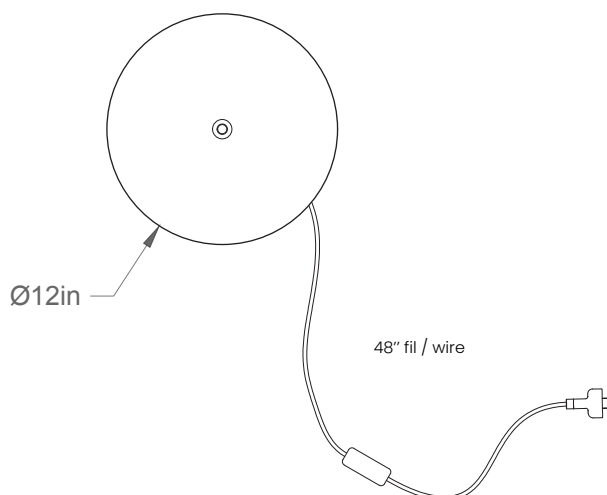
Dessus/Top
